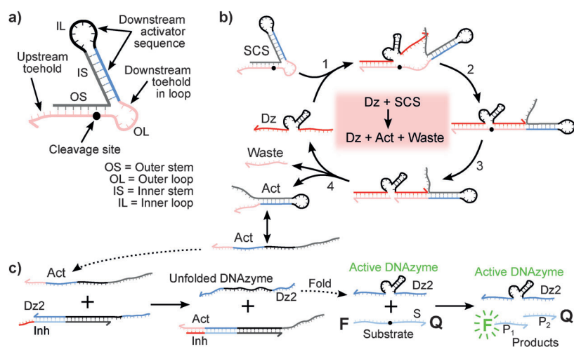
Figure 1. SCS design and mechanisms for SCS cleavage and DNAzyme displacement.
